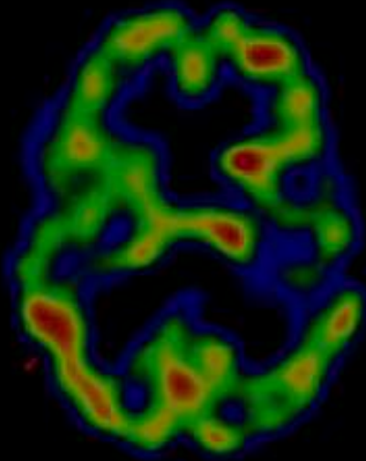
Baseline Scan
