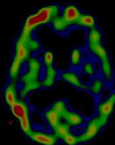
Prayer Scan
